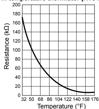
Fin temperature thermistor (RT64)
