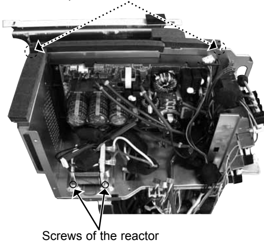
Screws of the outdoor power P.C. board
